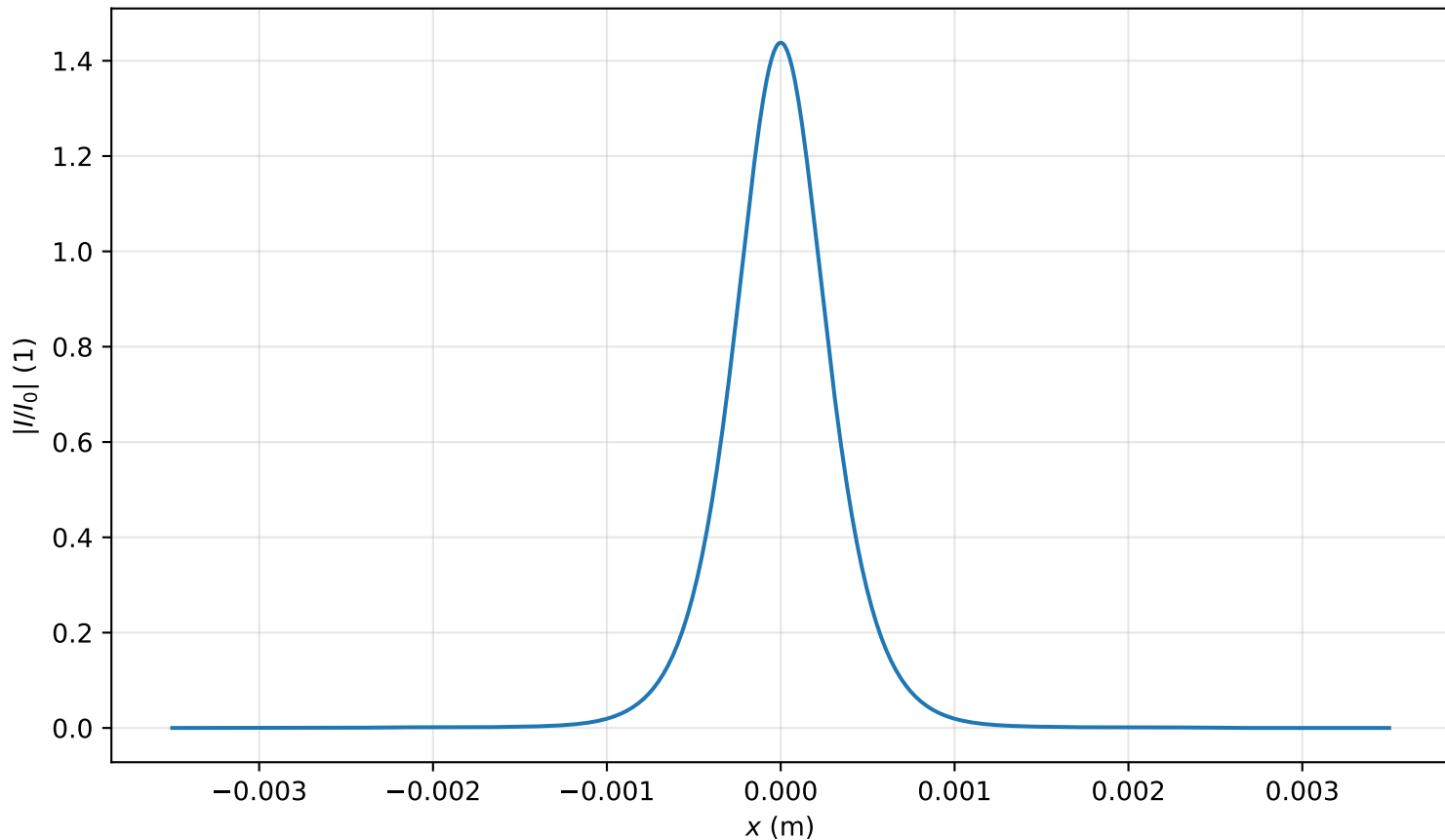
Intensity profile I(x, y = 0, z = 3.821m)/I_0 , P_{in}=0.9P_{cr} , artificial time
